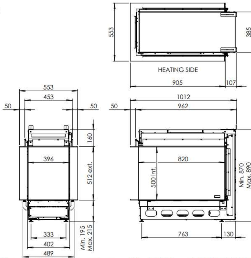
Dimensional Drawing e-Matrix heat 800x500 RD (MkII)
